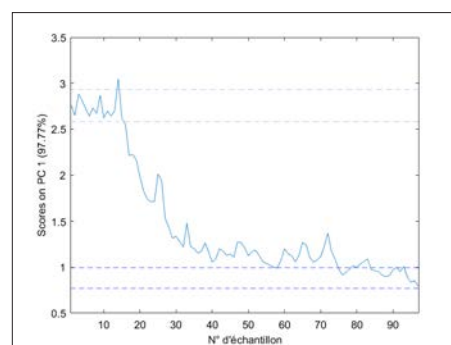
Figure 4: Monitoring of transition between two products (7 to 3) by means of the absorbance spectral
