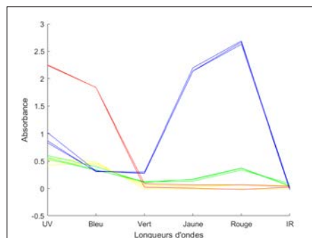
Figure 3: Transmission absorbance spectra of the detergents
